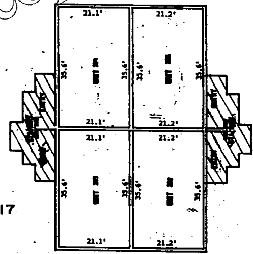
SECOND FLOOR PLAN (TYPICAL)
